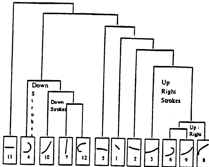
Figure 11: Hierarchical (Density linkage) clustering of the 12 pen-strokes of the same writer
